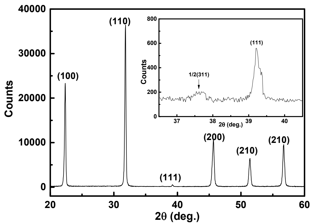
Fig. S1 Room temperature XRD pattern of (\text{Na}_{0.52}\text{K}_{0.4})(\text{Nb}_{0.84}\text{Sb}_{0.08})\text{O}_3-(0.08-x)\text{LiTaO}_3-x\text{BaZrO}_3 sample with x=0.04 .
